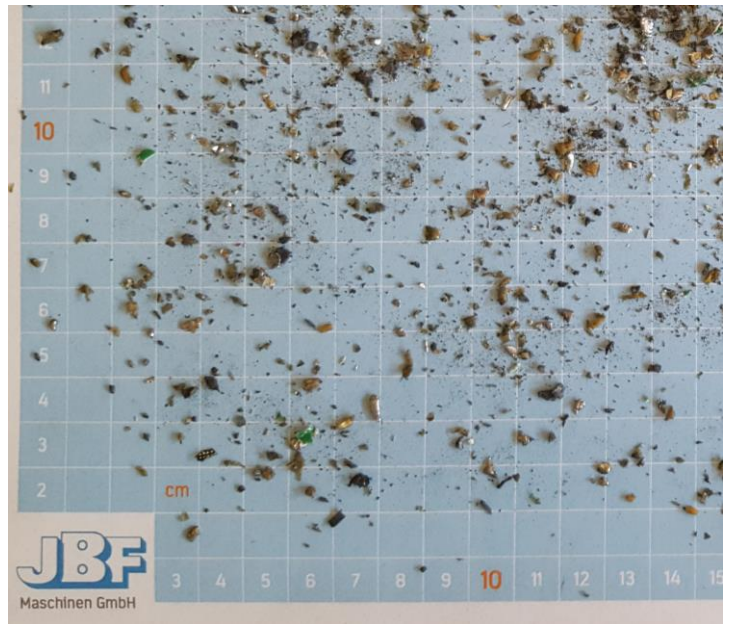
Cutting result FLASH 4 mm screen
